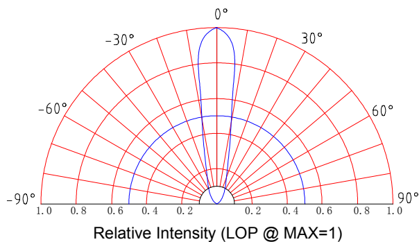
Beam Pattern
