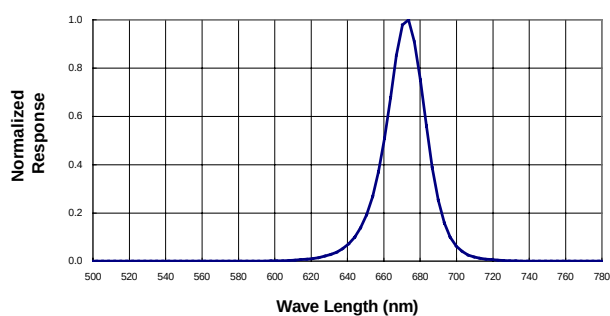
Spectral Radiance ( Peak @ 676nm)
