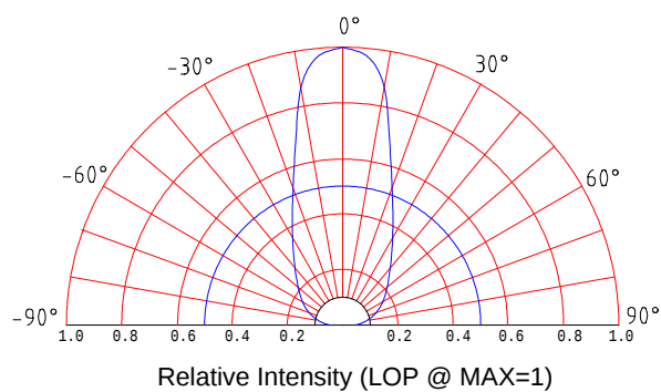
Beam Pattern
