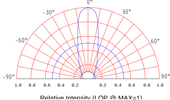
Beam Pattern
