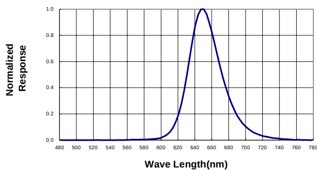
Spectral Radiance (Peak @ 644nm)
