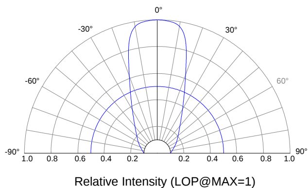
Beam Pattern
