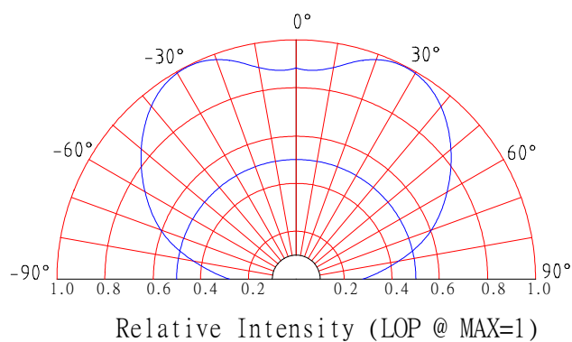
Beam Pattern
