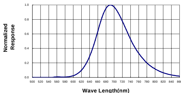
Spectral Radiance (Peak @ 700nm)
