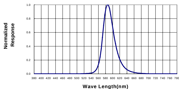
Spectral Radiance (Peak @ 588nm)
