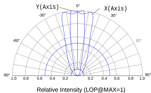
Beam Pattern
