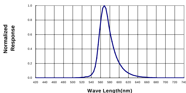
Spectral Radiance (Peak @ 568nm)
