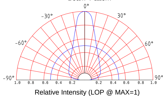
Beam Pattern
