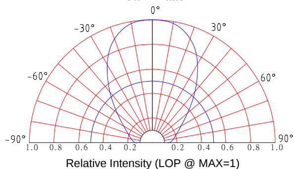
Beam Pattern
