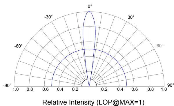
Beam Pattern
