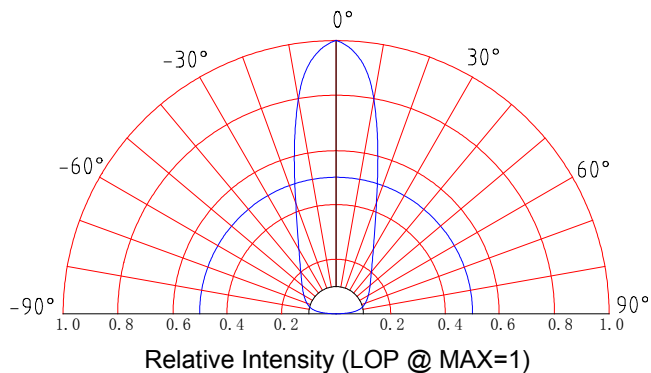
Beam Pattern
