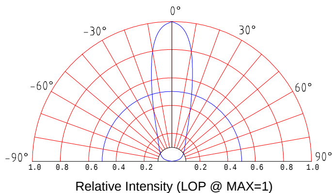
Beam Pattern
