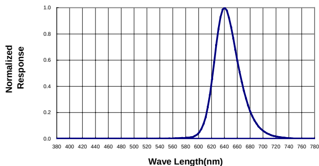
Spectral Radiance (Peak @ 640nm)
