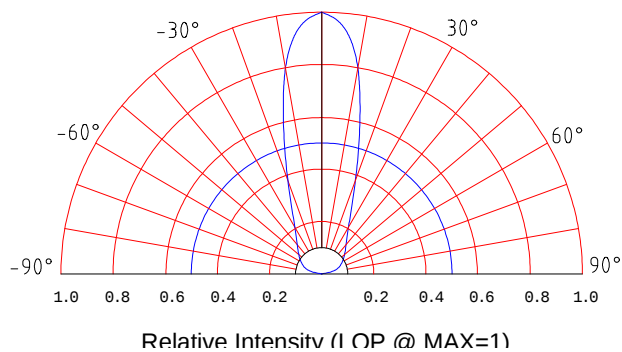
Beam Pattern
