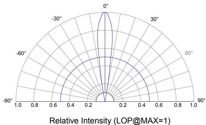
Beam Pattern
