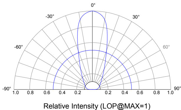
Beam Pattern
