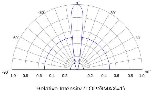
Beam Pattern
