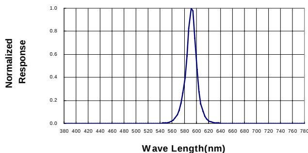
Spectral Radiance (Peak @ 593nm)
