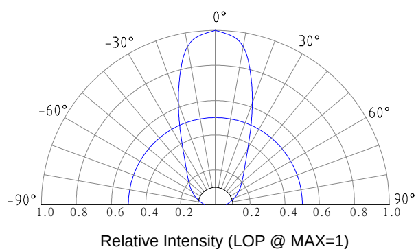
Beam Pattern
