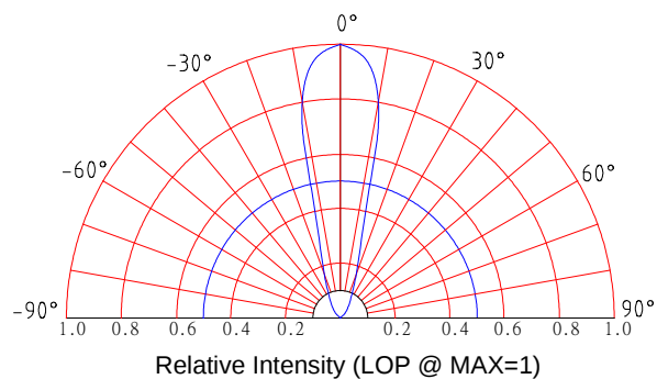
Beam Pattern
