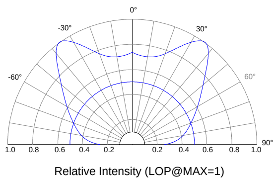
Beam Pattern
