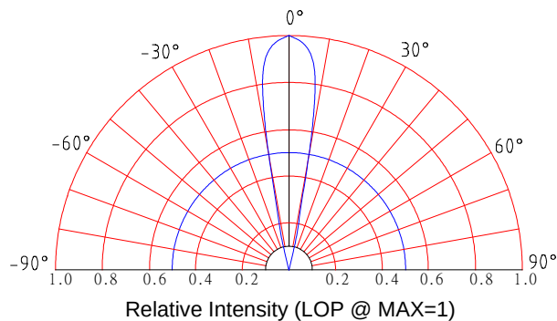
Beam Pattern
