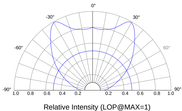
Beam Pattern
