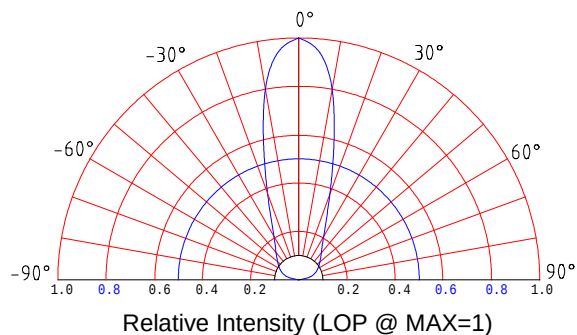
Beam Pattern
