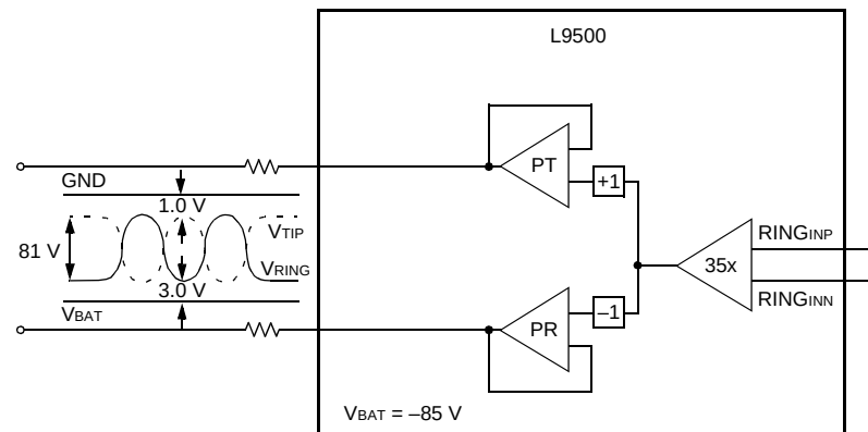
Figure 11. RINGIN Operation
