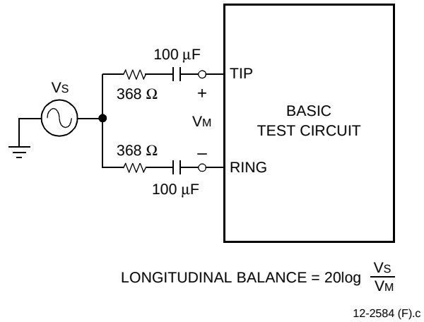
Figure 7. Longitudinal Balance
