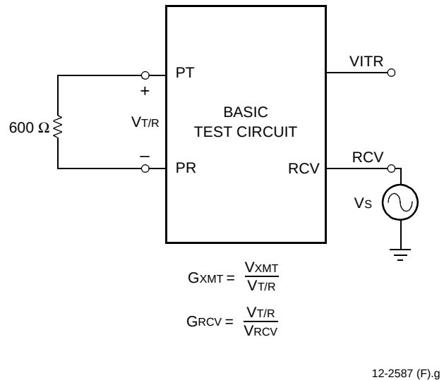
Figure 8. ac Gains
