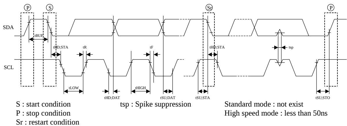
Figure 8 IIC timing
