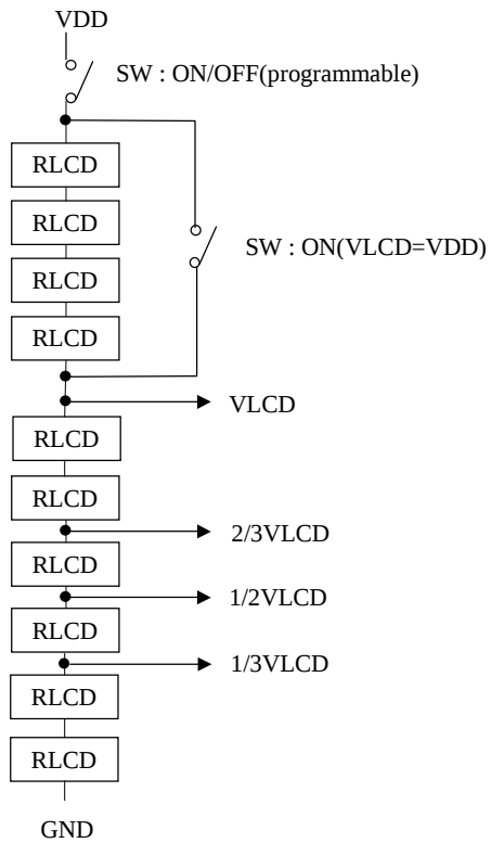
Figure 8 LCD bias resistor
