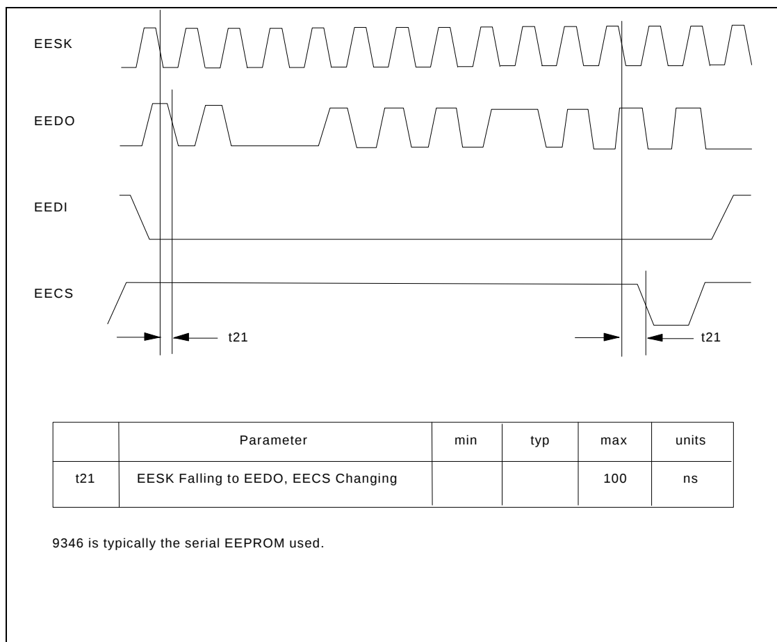
FIGURE 37 - EEPROM WRITE
