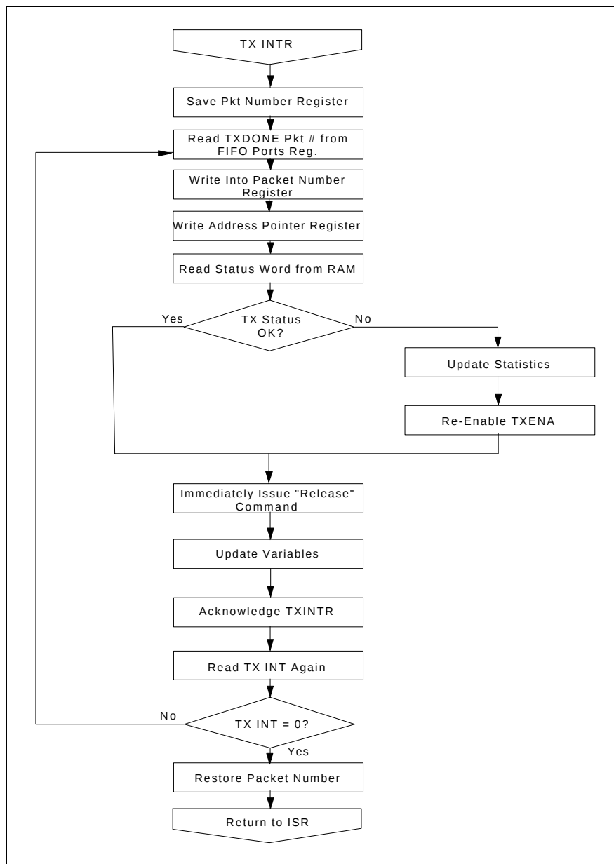
FIGURE 13 - TX INTR (Assumes Auto Release Option Selected)
