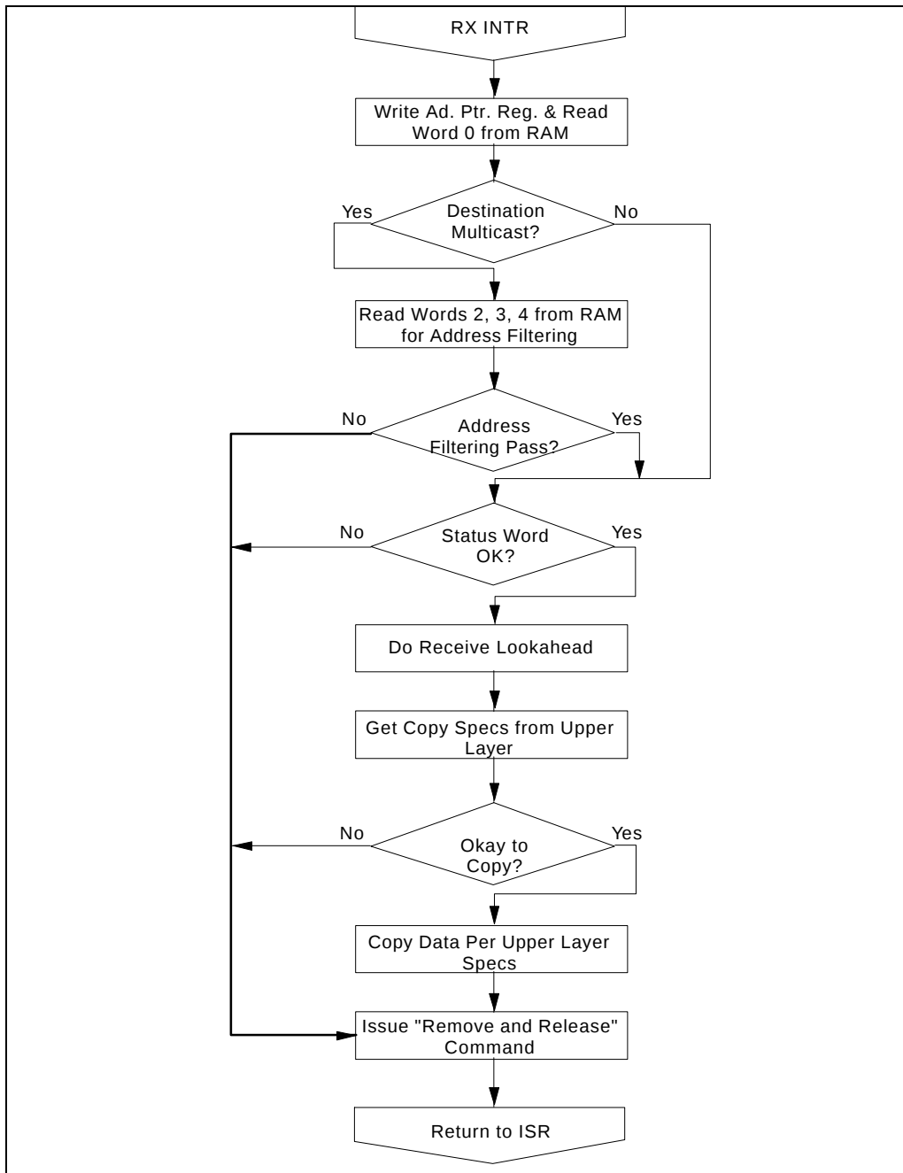
FIGURE 12 - RX INTR
