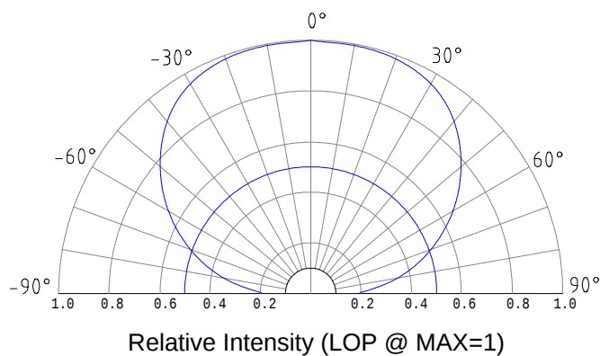
Beam Pattern
