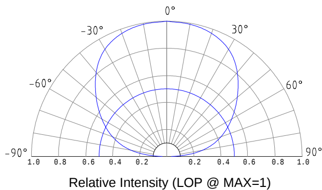
Beam Pattern
