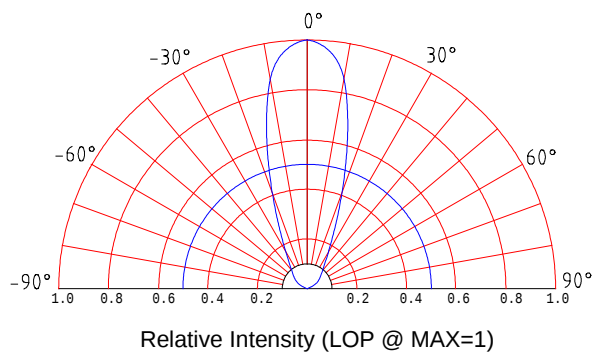
Beam Patter
