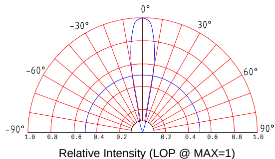
Beam Pattern
