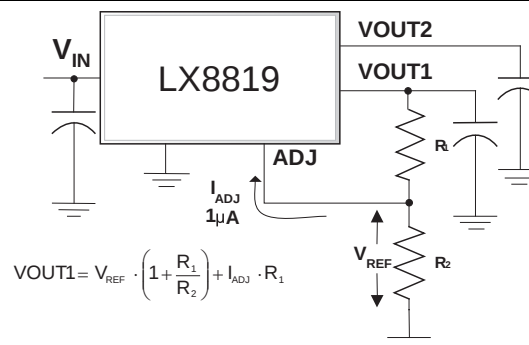
Figure 2 – Basic Regulator Circuit
