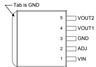
DF PACKAGE (Top View)
