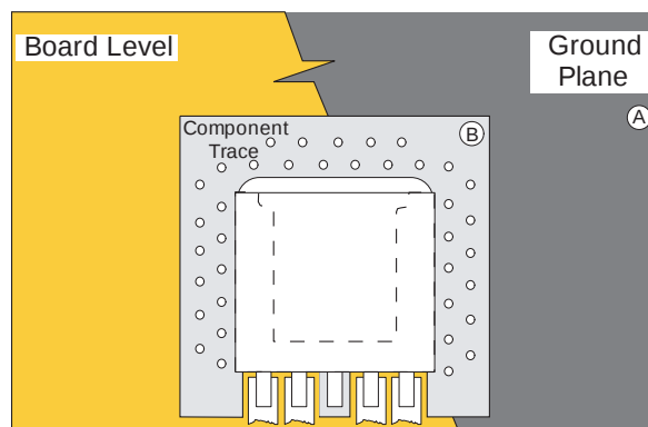
Figure 3 – Recommended Layout
