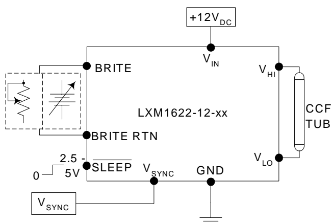
Figure 5 - Brightness Control
