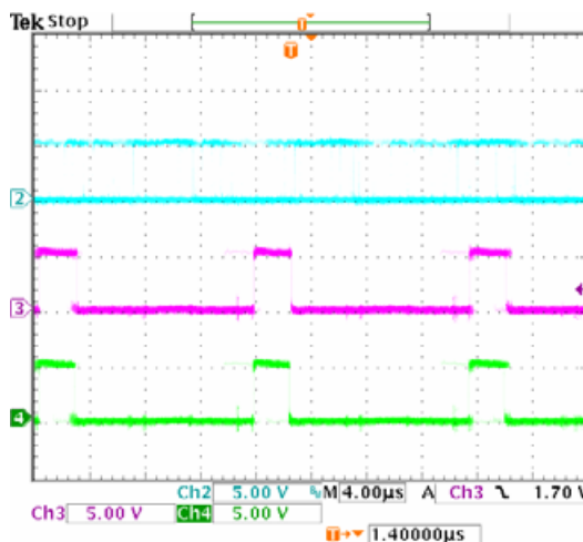
Figure 5- Master is in striking mode while slaves are in running mode CH2= A OUT (Master), CH3=A OUT (Slave1), CH4=A OUT (Slave2)
