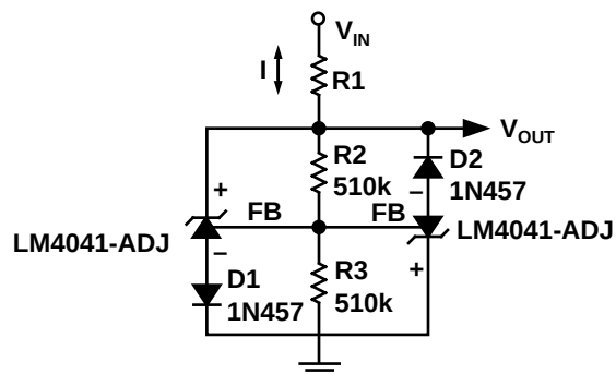
Figure 6. Bidirectional Clamp +2.4V
