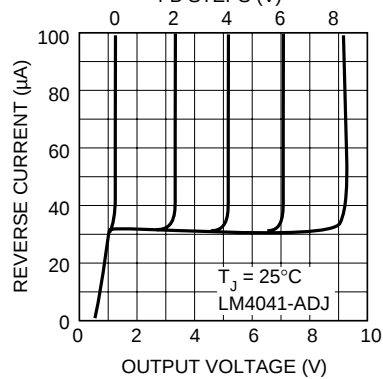
Reverse Characteristics †
