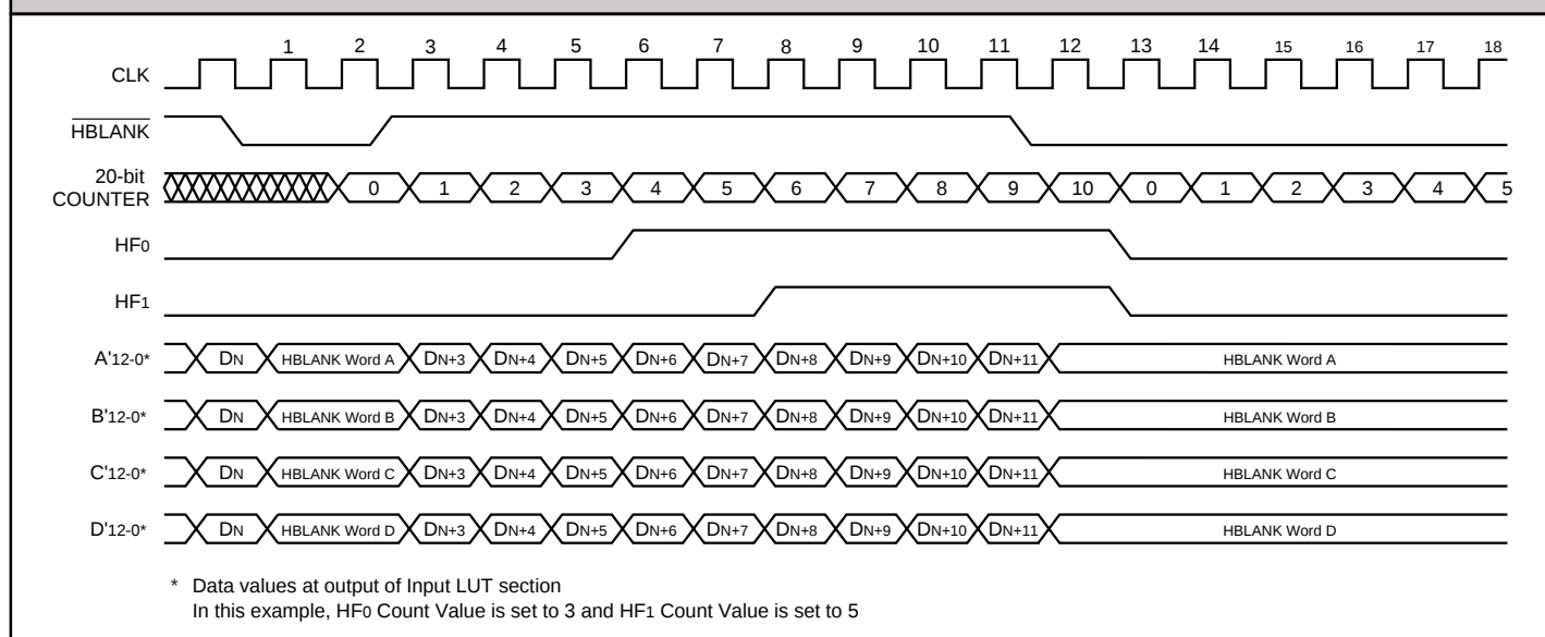
FIGURE 10. \overline{\text{HBLANK}} AND COUNTER
