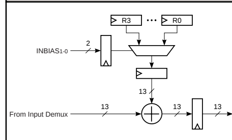
FIGURE 8. INPUT BIAS
