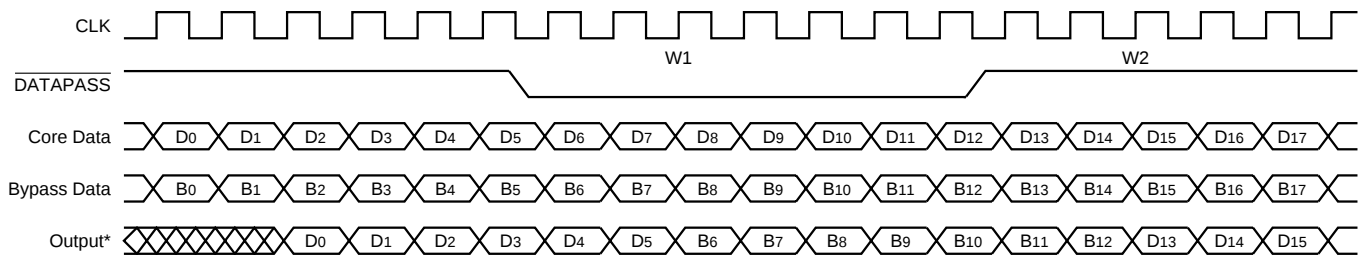
FIGURE 16. CORE BYPASS
