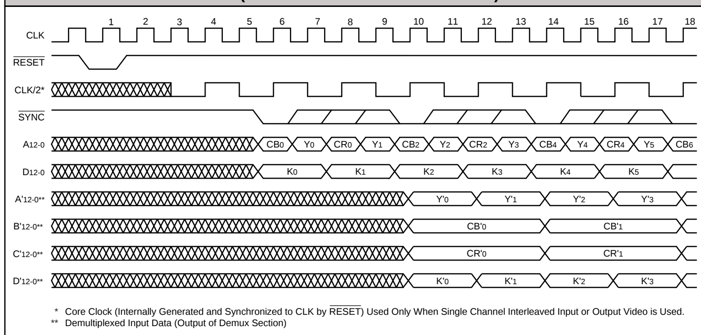
FIGURE 5. INPUT PROCESSING 4:2:2:4 (INTERLEAVED LUMA/CHROMA ON CHANNEL A)
