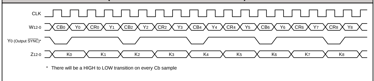
FIGURE 7. OUTPUTTING 4:2:2:4 (INTERLEAVED LUMA/CHROMA ON CHANNEL W)
