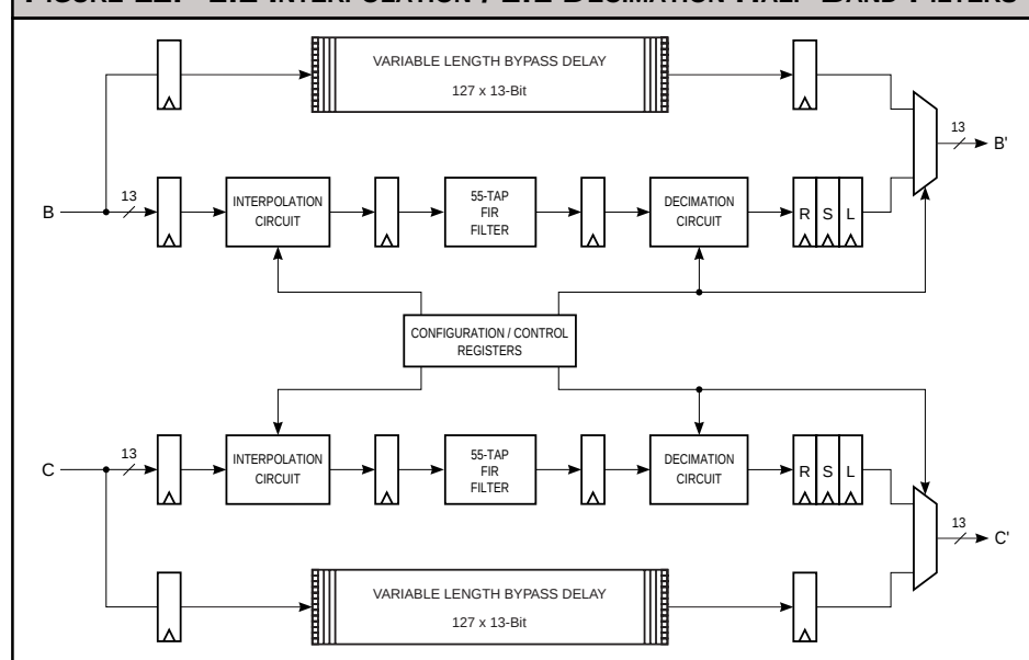
FIGURE 12. 1:2 INTERPOLATION / 2:1 DECIMATION HALF-BAND FILTERS
