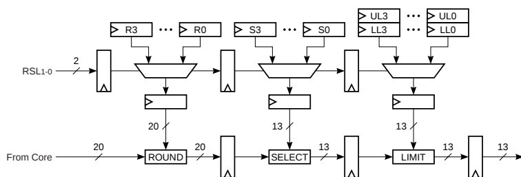
FIGURE 13. RSL CIRCUITRY
