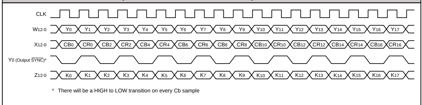
FIGURE 6. OUTPUTTING 4:2:2:4 (INTERLEAVED CHROMA ON CHANNEL X)
