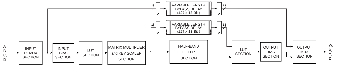
FIGURE 15. BYPASS BLOCK DIAGRAM
