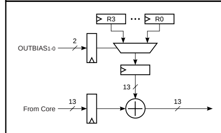
FIGURE 9. OUTPUT BIAS
