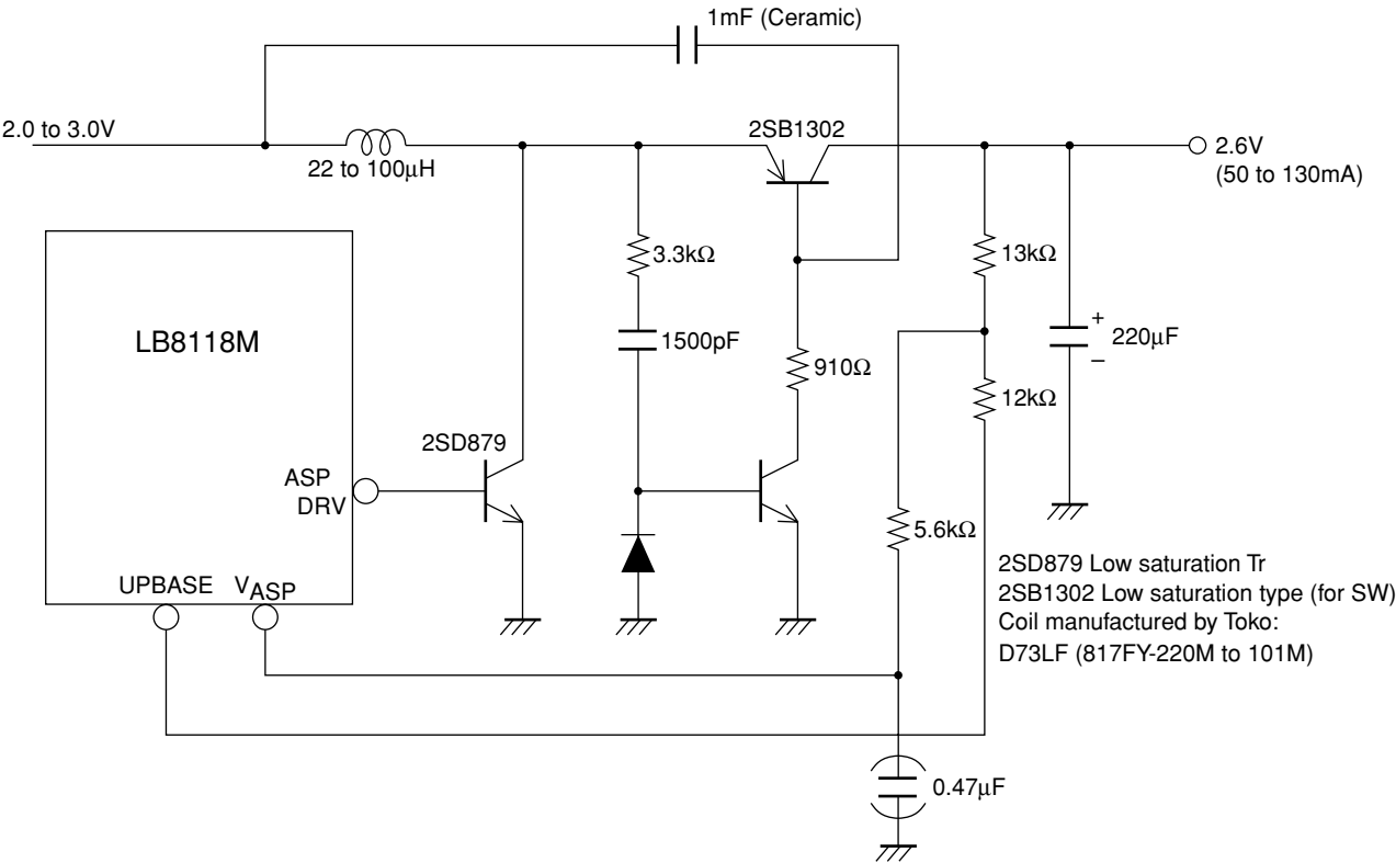
Figure 1 DC 2.6 V Up/down Sample Application 1
