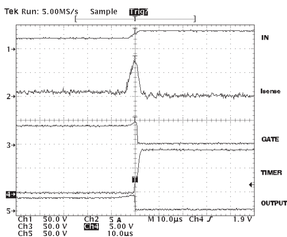
Figure 13. Overvoltage Waveforms
