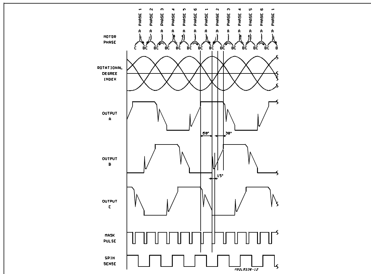
Figure 4-1: Waveforms
