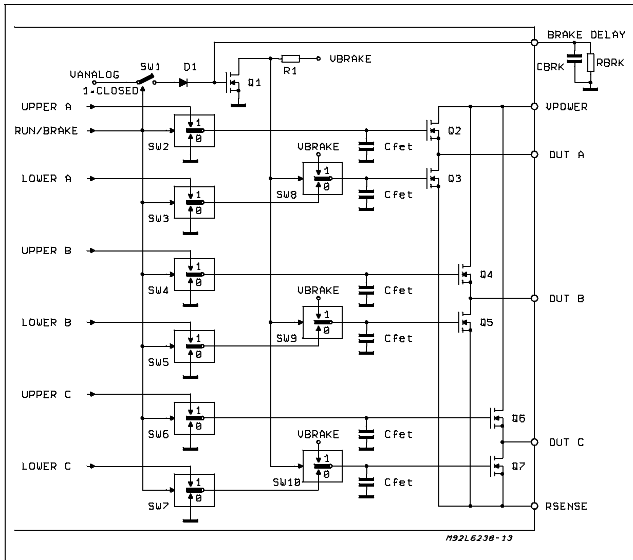
Figure 16: Brake Delay.
