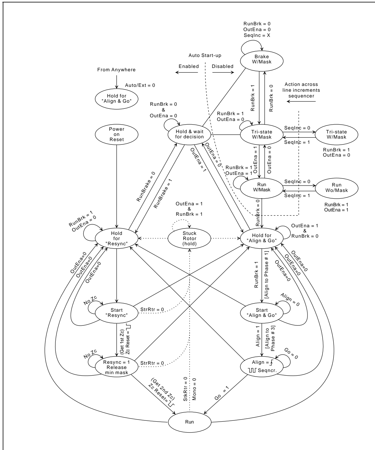
Figure 4: State Diagram
