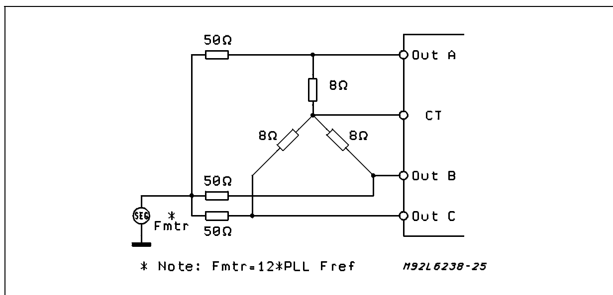
Figure 28: Bemf Emulator.
