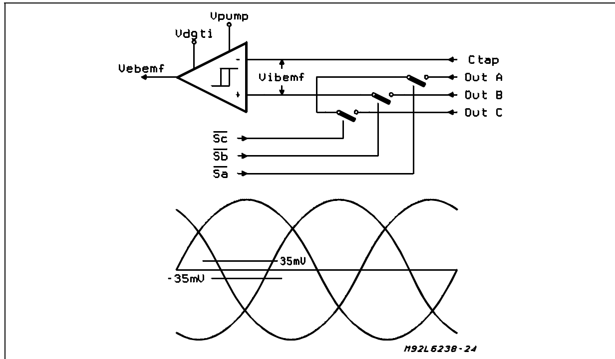
Figure 27: Bemf Amplifier.
