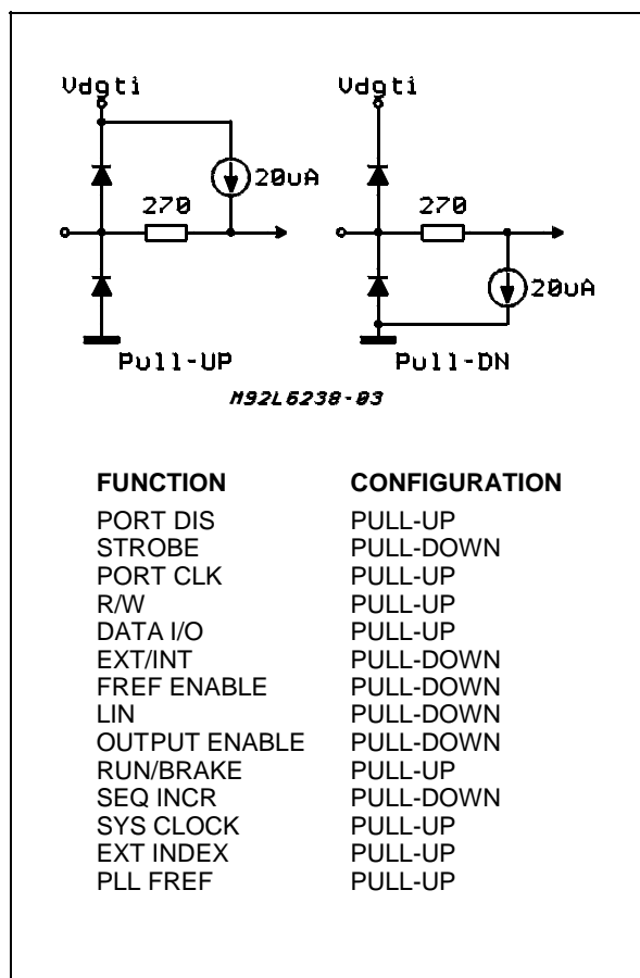
Figure 2: Input Structures
