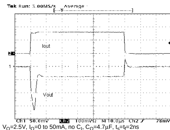
Figure 14 : Load Transient
