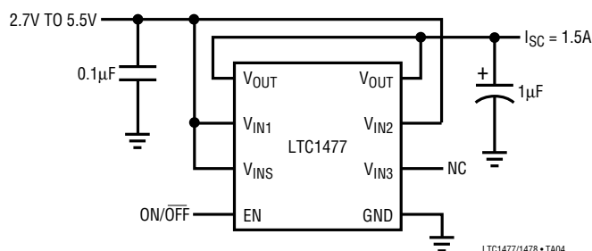
1.5A Protected Switch
