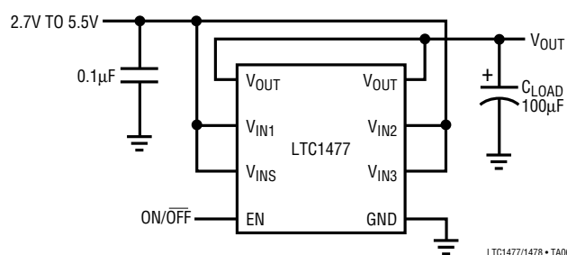
2A Protected Switch Driving a Large Capacitive Load
