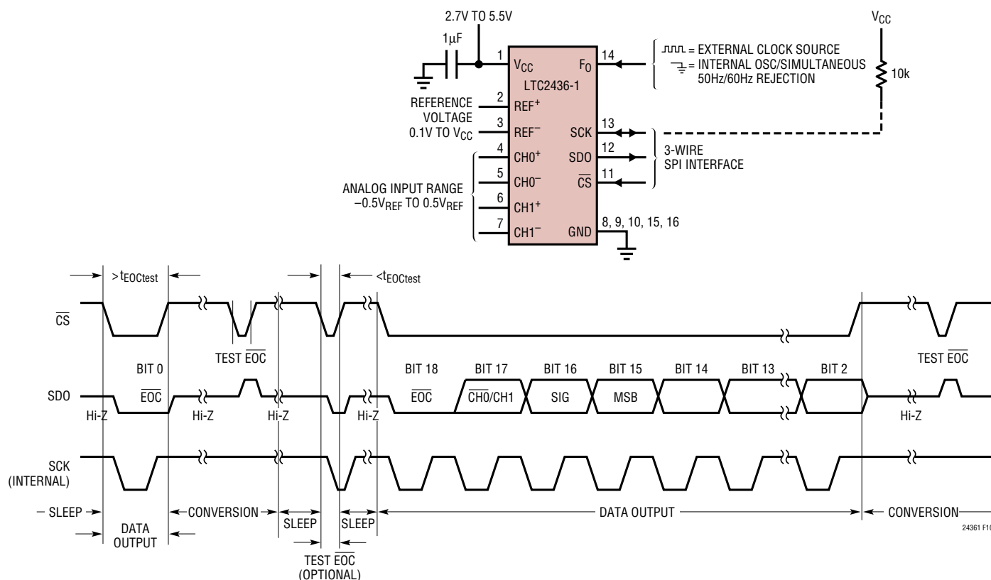
Figure 10. Internal Serial Clock, Reduced Data Output Length
