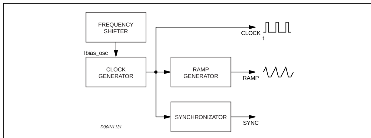
Figure 3. Oscillator Circuit
