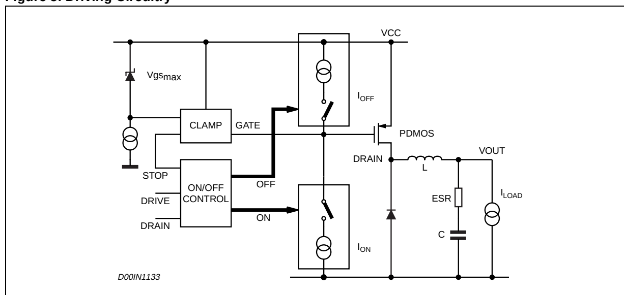
Figure 5. Driving Circuitry
