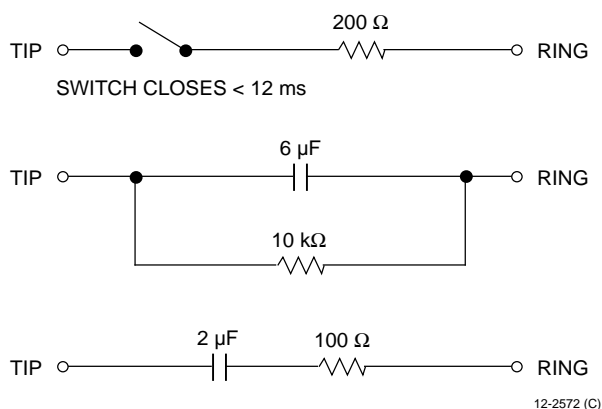
Figure 10. Ring-Trip Circuits
